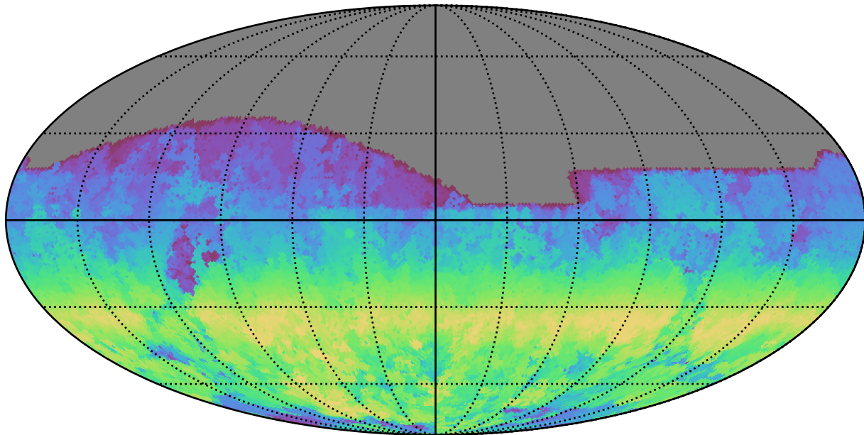
noroll_mjdp180_v3.4_10yrs All sky g band: AngleRange rotSkyPos
