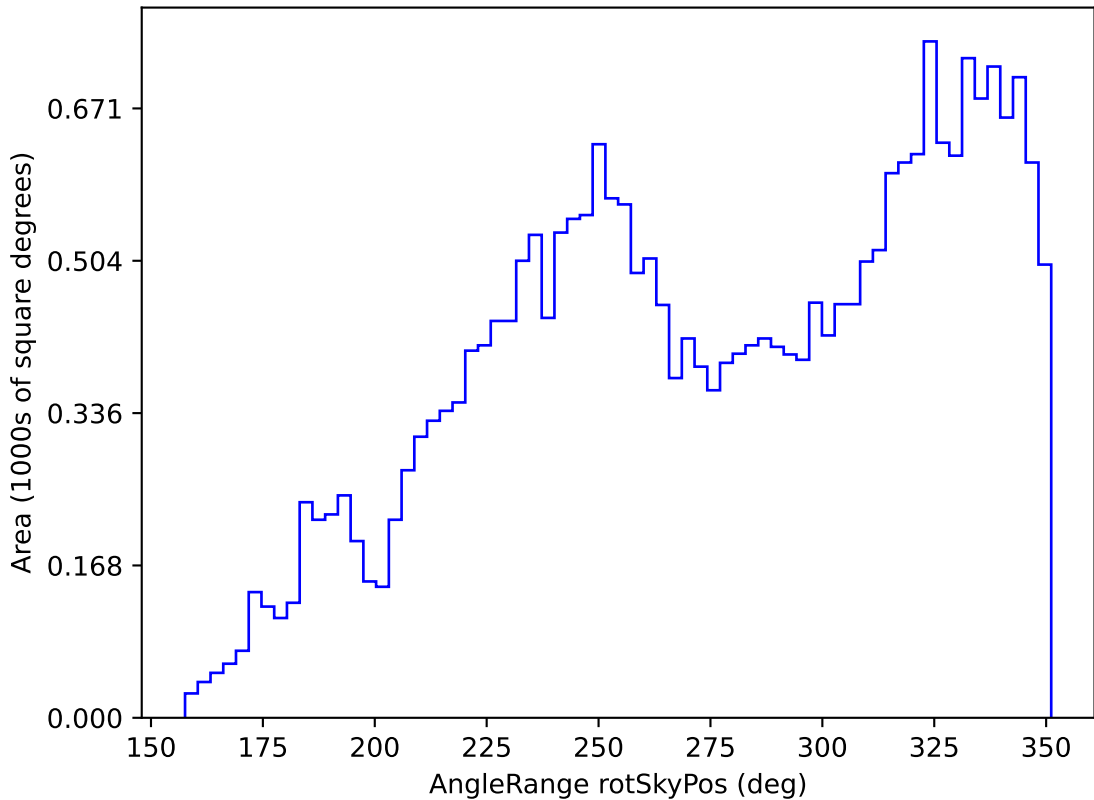
noroll_mjdp180_v3.4_10yrs All sky all bands: AngleRange rotSkyPos
