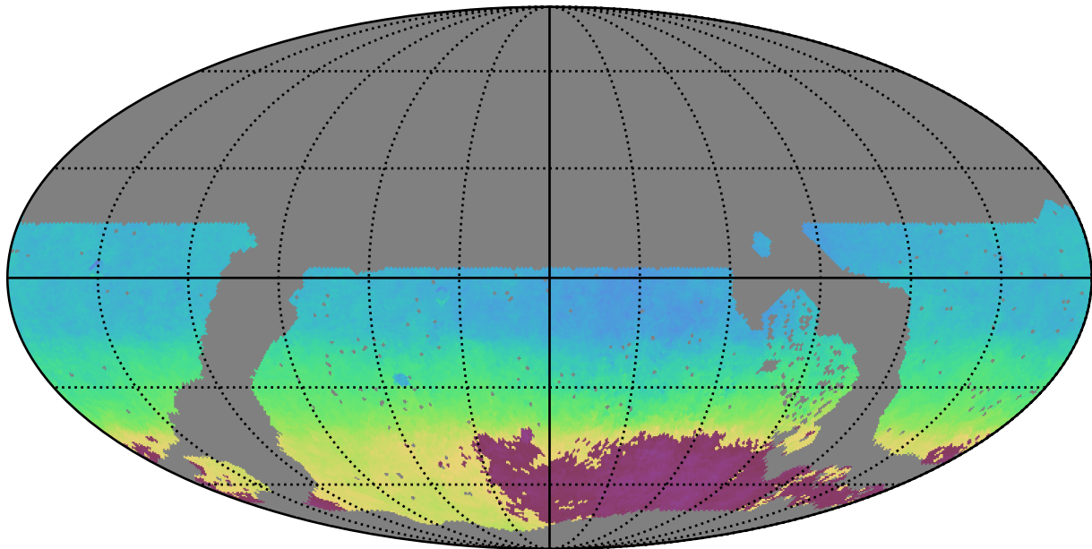
noroll_mjdp180_v3.4_10yrs WFD y band: AngleMean rotSkyPos
