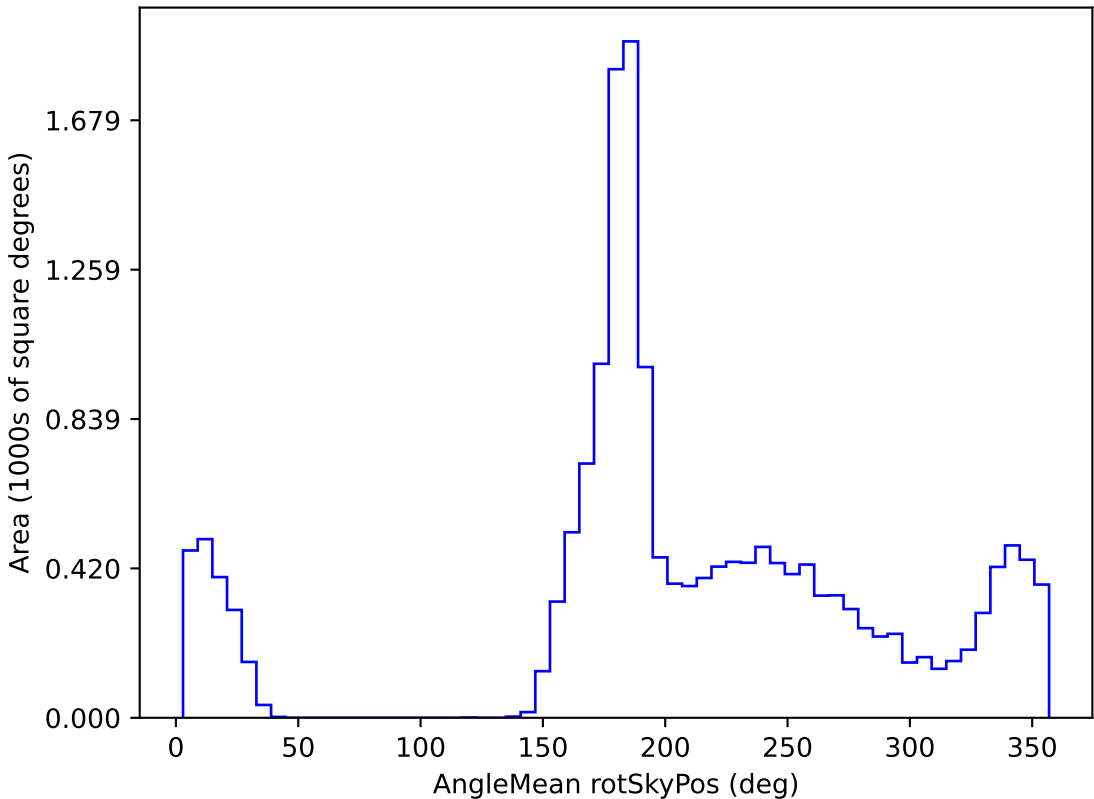
noroll_mjdp180_v3.4_10yrs WFD y band: AngleMean rotSkyPos
