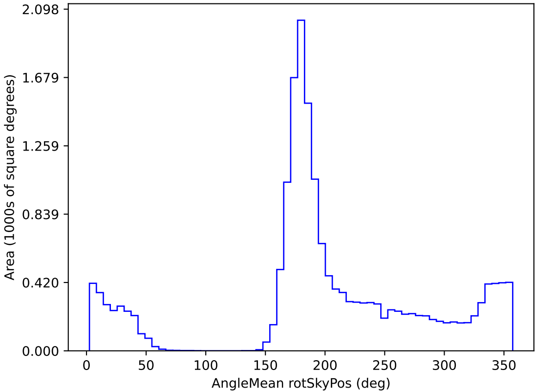
noroll_mjdp180_v3.4_10yrs WFD u band: AngleMean rotSkyPos
