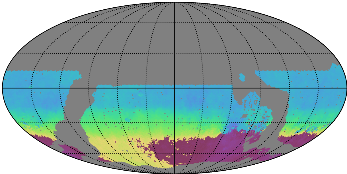
noroll_mjdp180_v3.4_10yrs WFD r band: AngleMean rotSkyPos
