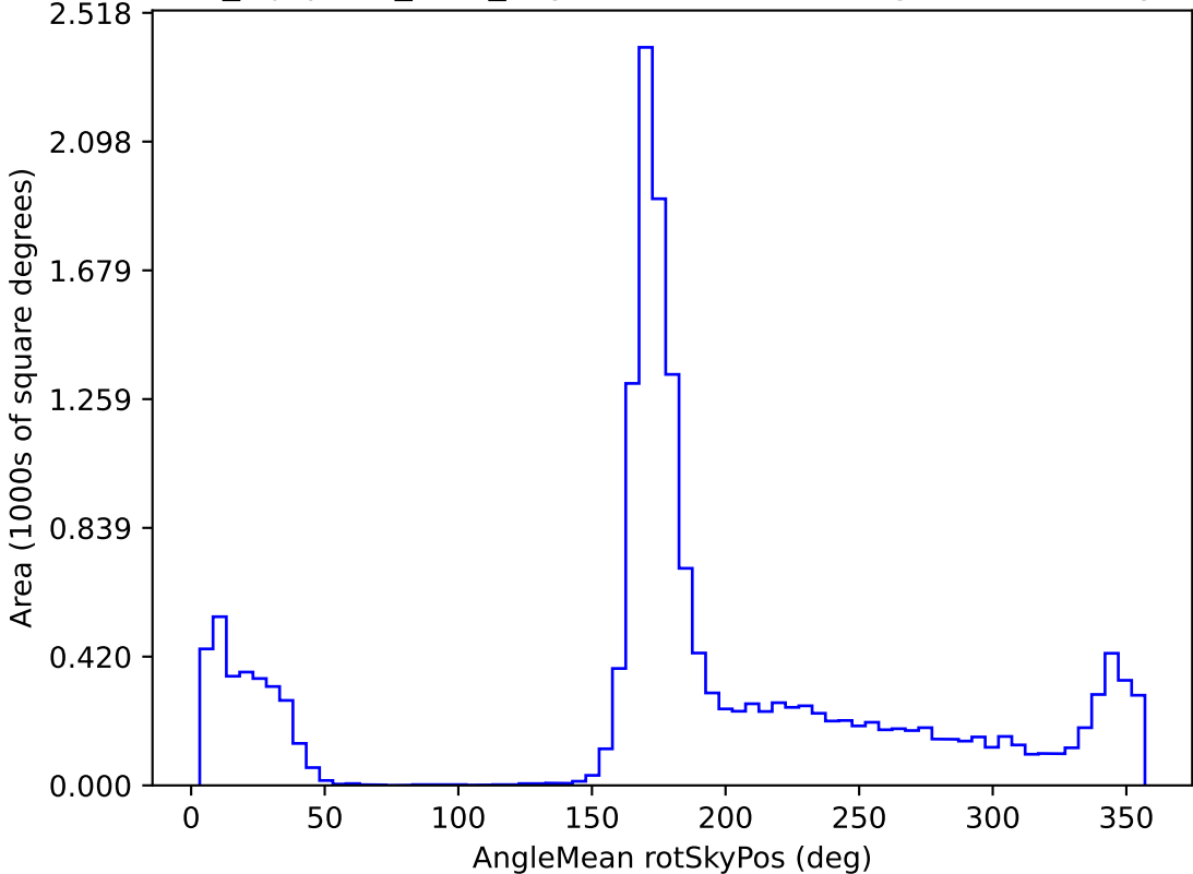
noroll_mjdp180_v3.4_10yrs WFD r band: AngleMean rotSkyPos
