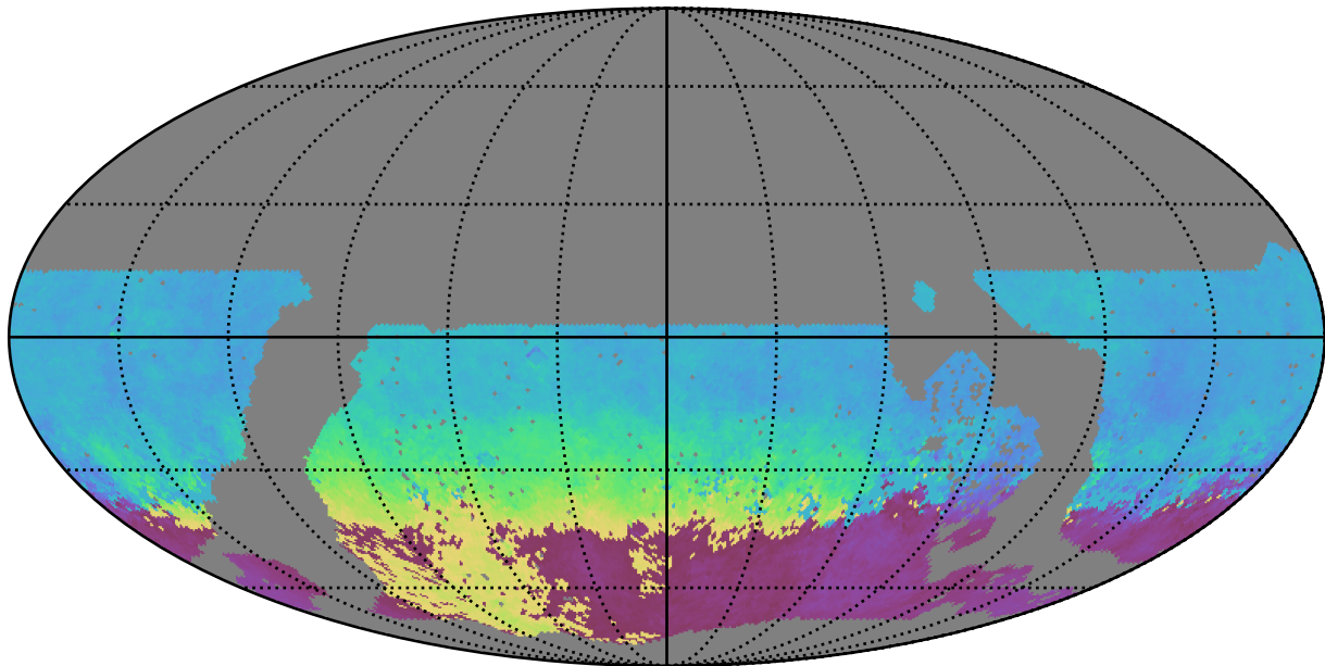
noroll_mjdp180_v3.4_10yrs WFD g band: AngleMean rotSkyPos
