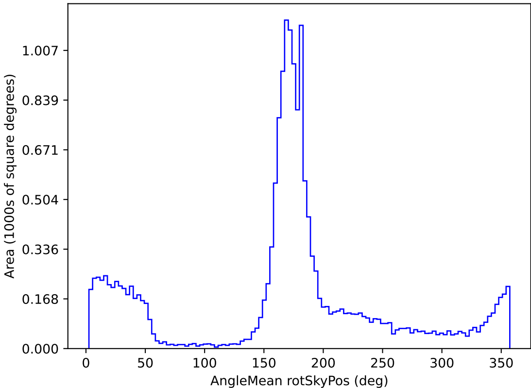
noroll_mjdp180_v3.4_10yrs WFD g band: AngleMean rotSkyPos
