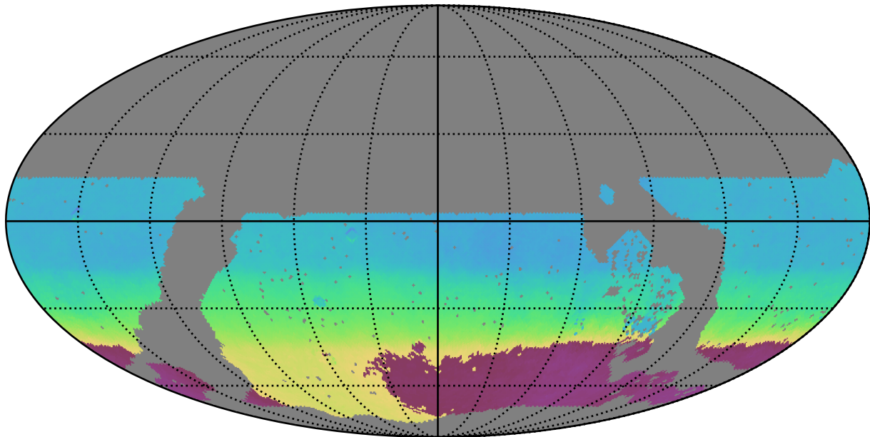
noroll_mjdp180_v3.4_10yrs WFD all bands: AngleMean rotSkyPos
