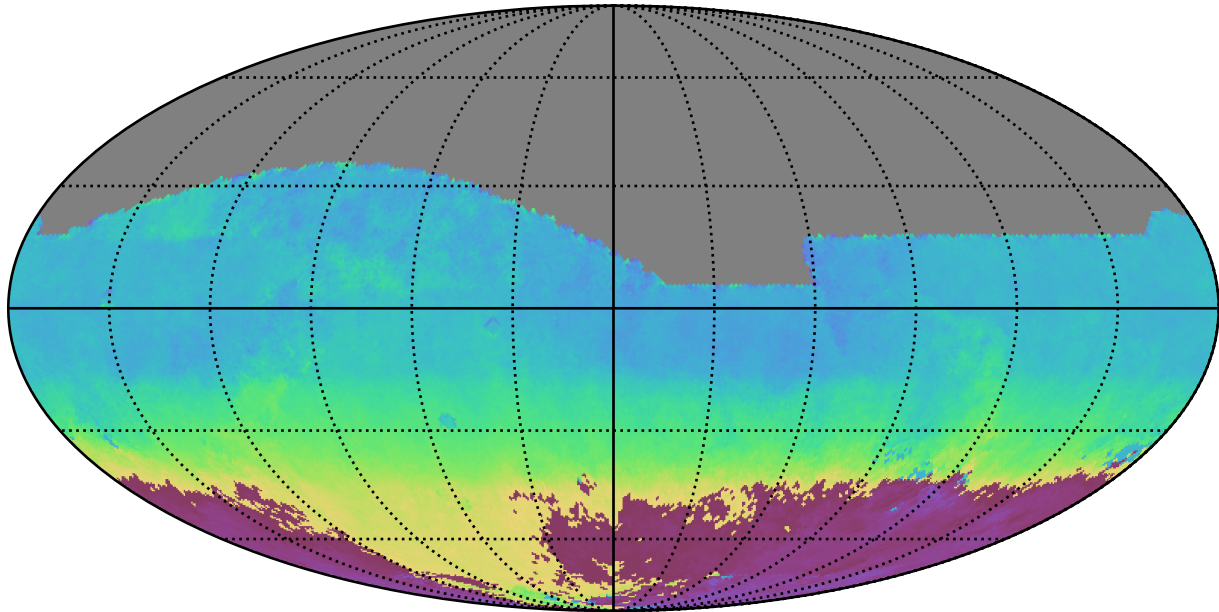
noroll_mjdp180_v3.4_10yrs All sky z band: AngleMean rotSkyPos
