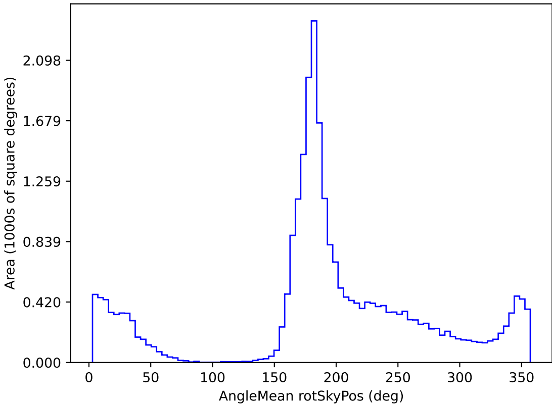
noroll_mjdp180_v3.4_10yrs All sky z band: AngleMean rotSkyPos
