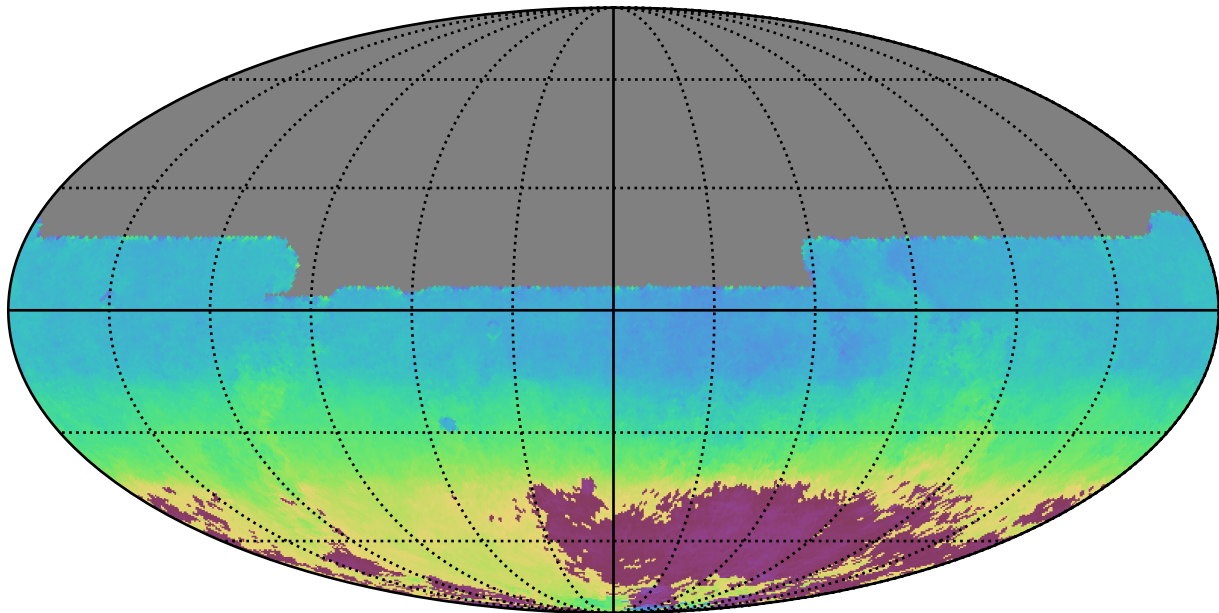
noroll_mjdp180_v3.4_10yrs All sky y band: AngleMean rotSkyPos
