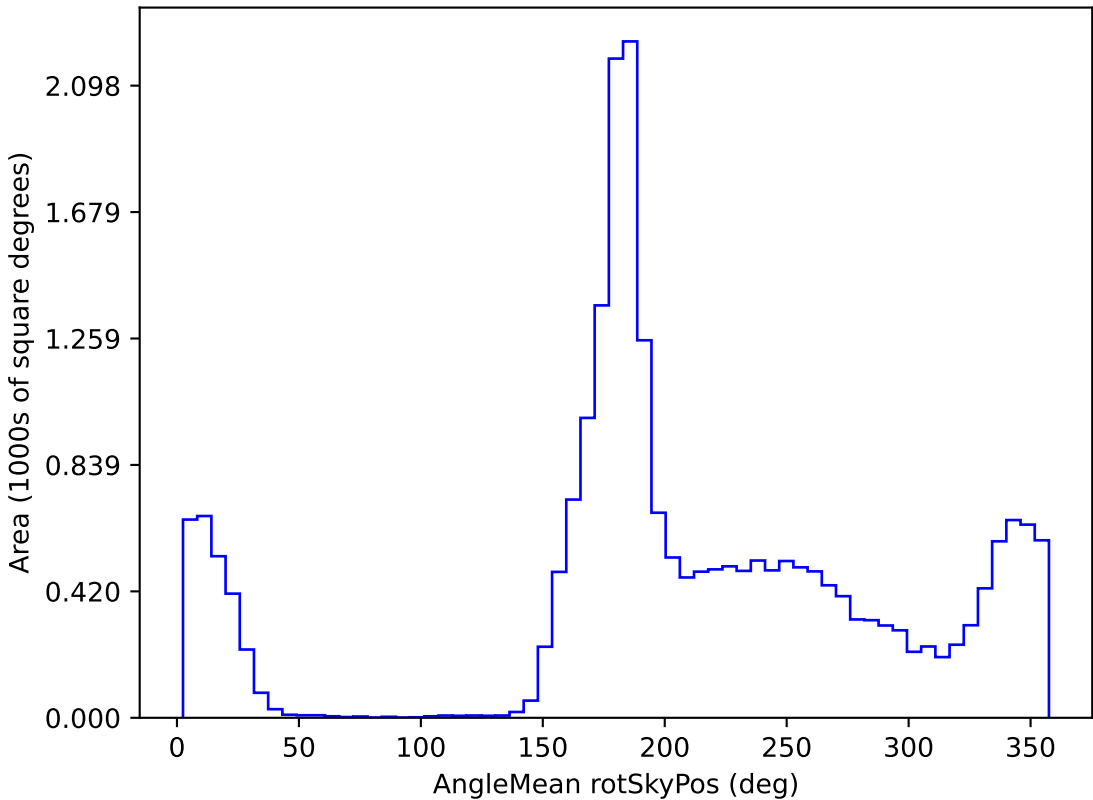
noroll_mjdp180_v3.4_10yrs All sky y band: AngleMean rotSkyPos
