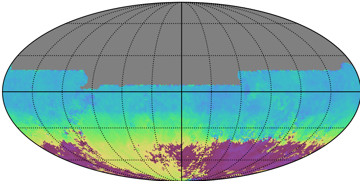
noroll_mjdp180_v3.4_10yrs All sky u band: AngleMean rotSkyPos
