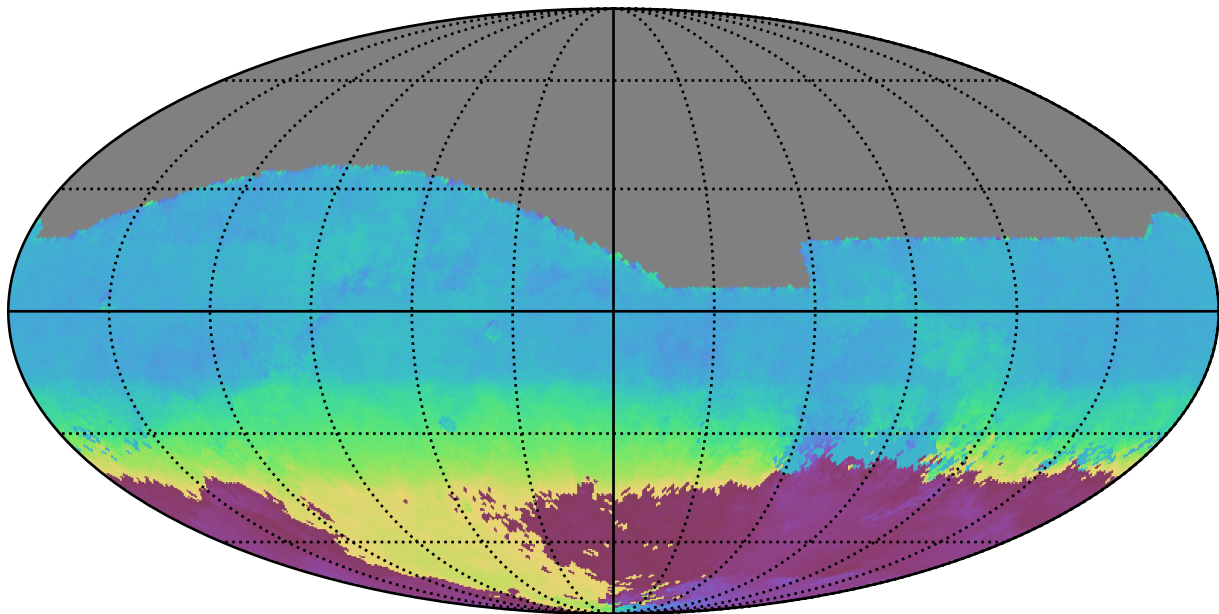
noroll_mjdp180_v3.4_10yrs All sky r band: AngleMean rotSkyPos
