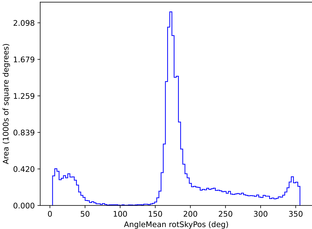
noroll_mjdp180_v3.4_10yrs All sky r band: AngleMean rotSkyPos
