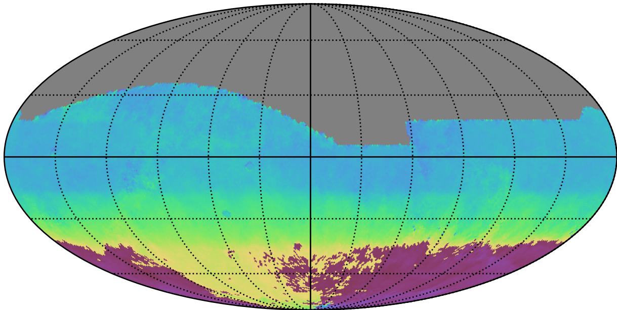
noroll_mjdp180_v3.4_10yrs All sky i band: AngleMean rotSkyPos
