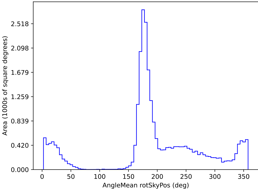
noroll_mjdp180_v3.4_10yrs All sky i band: AngleMean rotSkyPos
