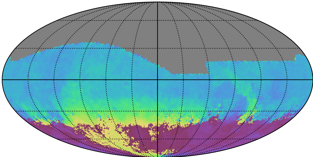
noroll_mjdp180_v3.4_10yrs All sky g band: AngleMean rotSkyPos
