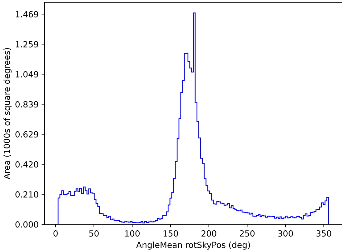
noroll_mjdp180_v3.4_10yrs All sky g band: AngleMean rotSkyPos
