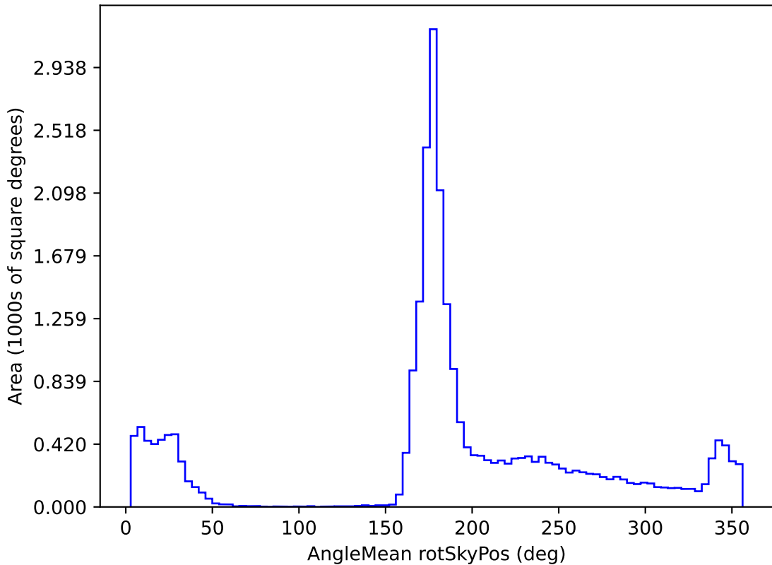
noroll_mjdp180_v3.4_10yrs All sky all bands: AngleMean rotSkyPos
