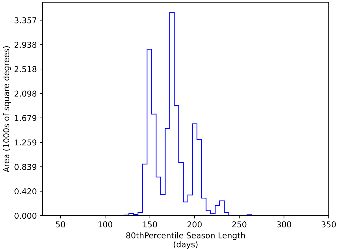
noroll_mjdp180_v3.4_10yrs WFD y band: 80thPercentile Season Length
