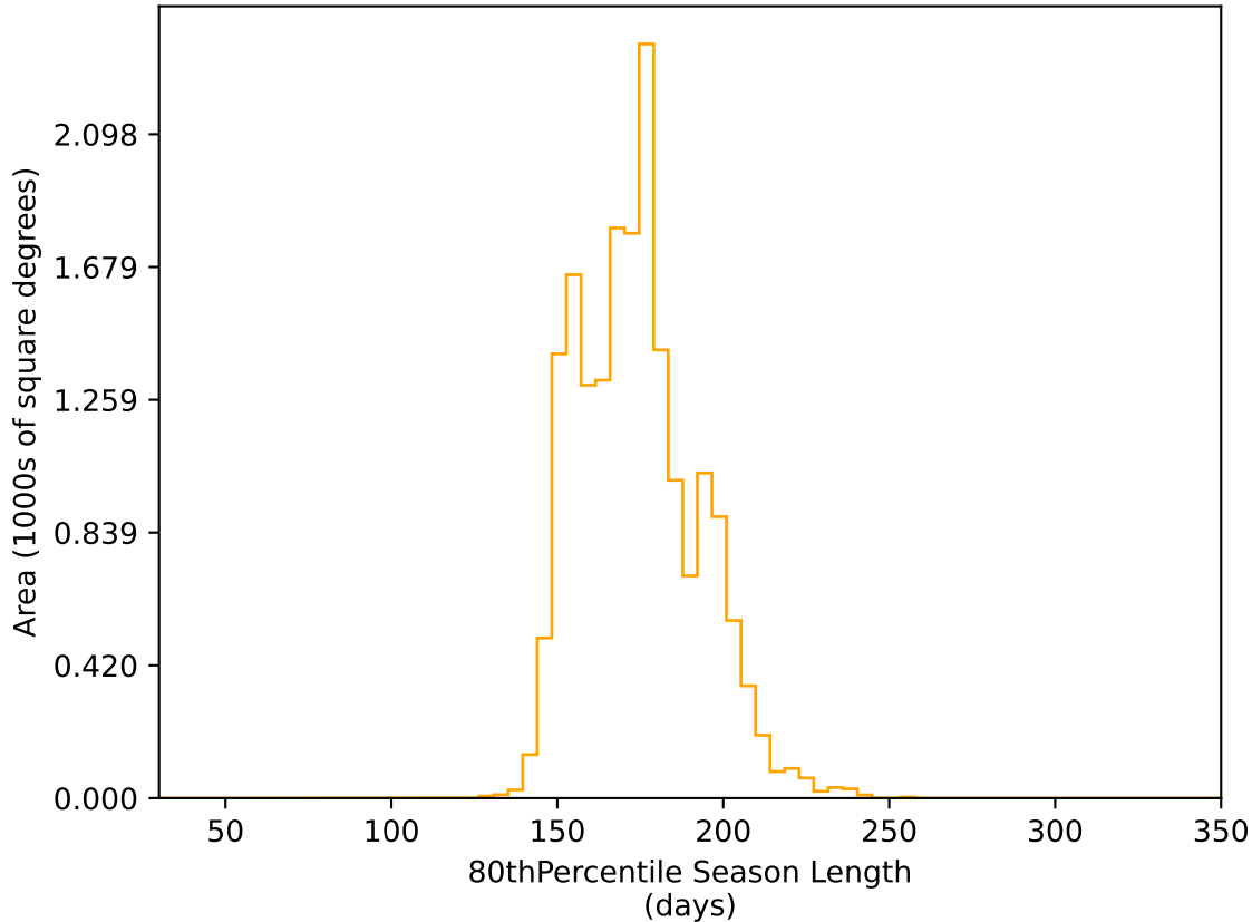
noroll_mjdp180_v3.4_10yrs WFD r band: 80thPercentile Season Length
