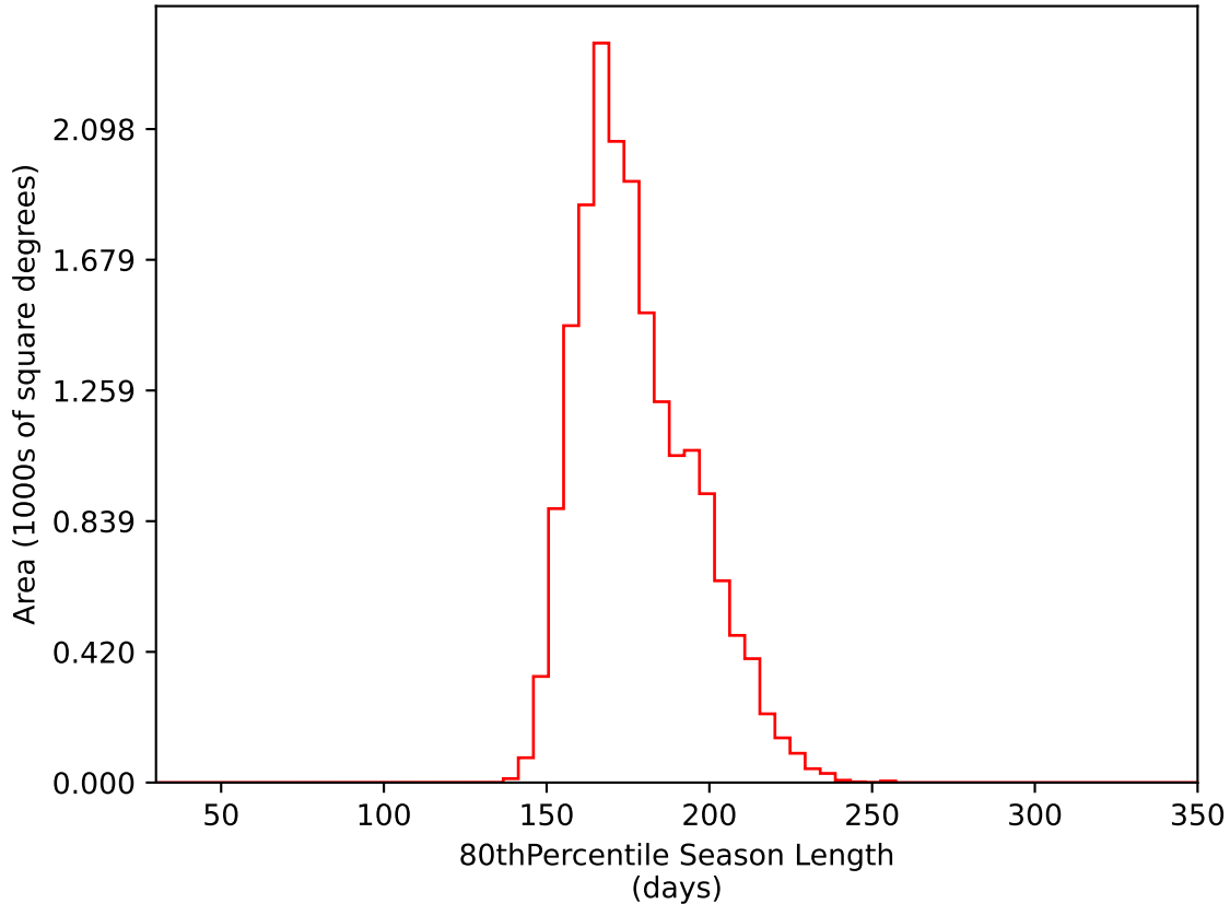
noroll_mjdp180_v3.4_10yrs WFD i band: 80thPercentile Season Length
