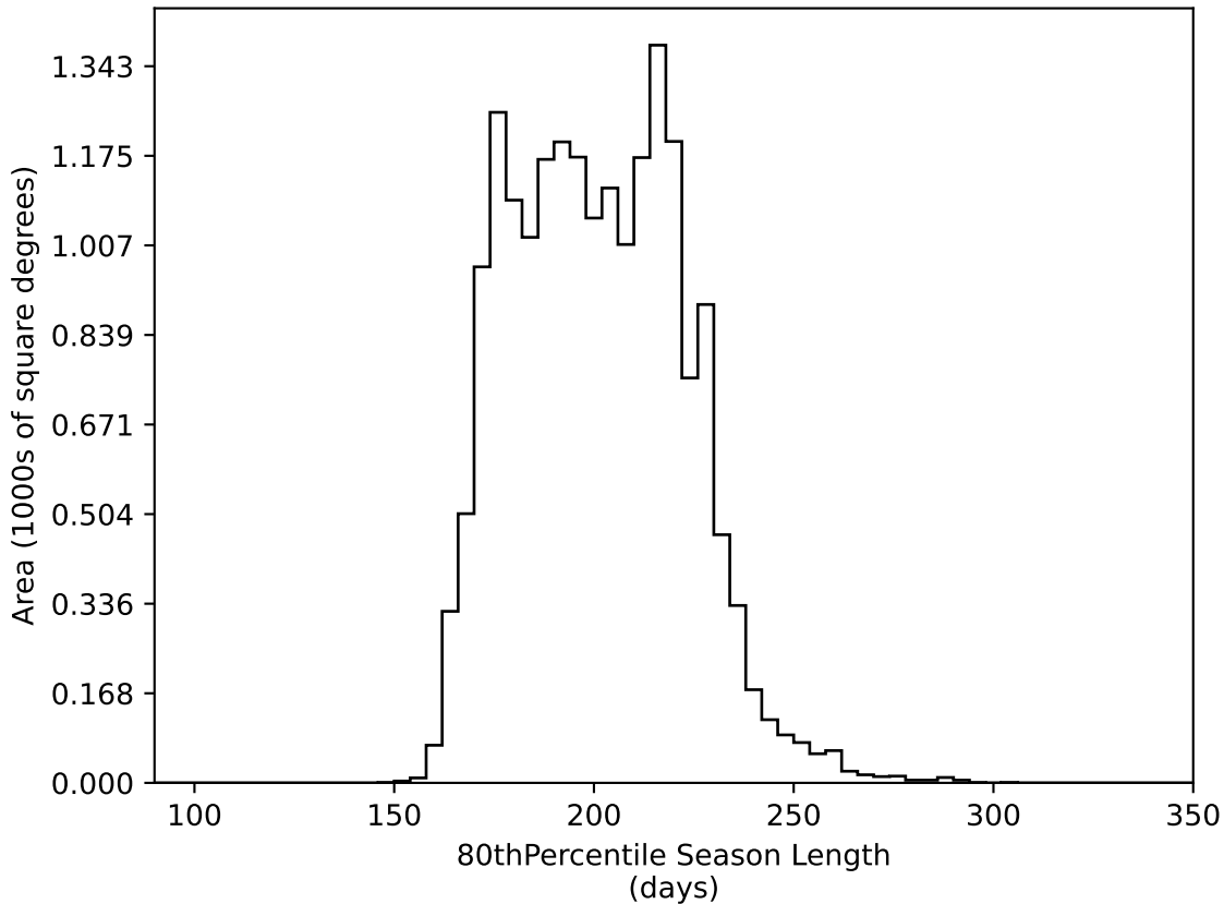
noroll_mjdp180_v3.4_10yrs WFD all bands: 80thPercentile Season Length
