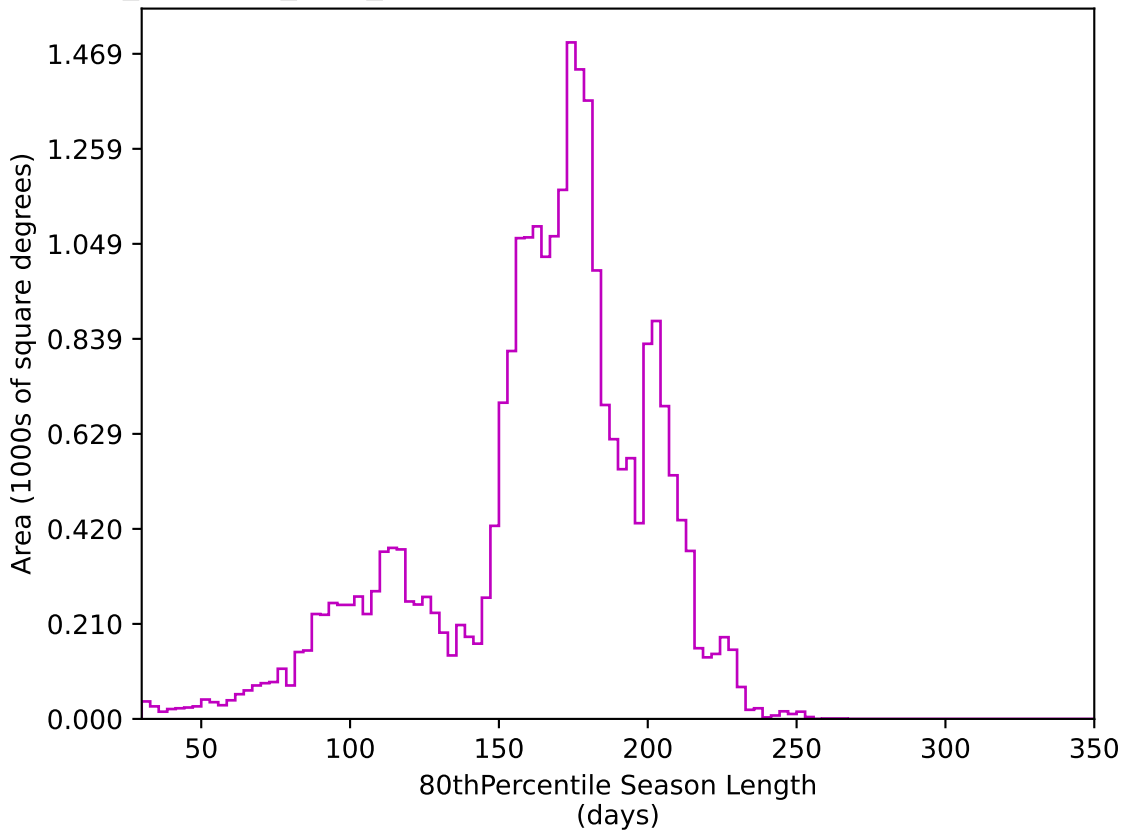
noroll_mjdp180_v3.4_10yrs All sky z band: 80thPercentile Season Length
