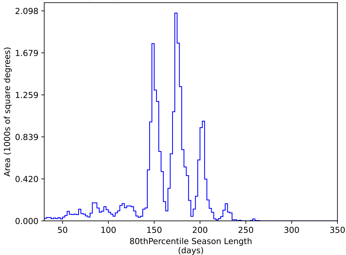
noroll_mjdp180_v3.4_10yrs All sky y band: 80thPercentile Season Length
