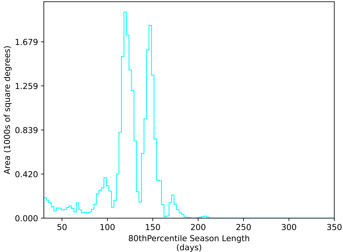
noroll_mjdp180_v3.4_10yrs All sky u band: 80thPercentile Season Length
