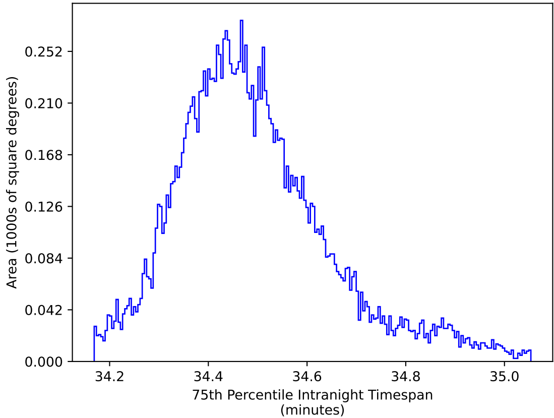
noroll_mjdp180_v3.4_10yrs WFD zy bands: 75th Percentile Intranight Timespan
