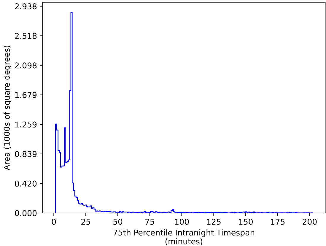
noroll_mjdp180_v3.4_10yrs WFD z band: 75th Percentile Intranight Timespan
