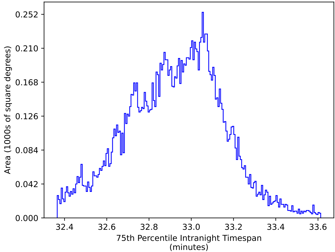
noroll_mjdp180_v3.4_10yrs WFD y band: 75th Percentile Intranight Timespan
