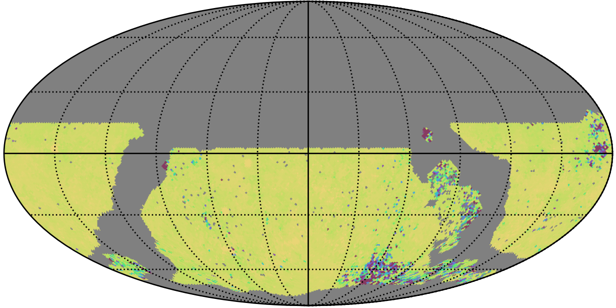
noroll_mjdp180_v3.4_10yrs WFD ug bands: 75th Percentile Intranight Timespan
