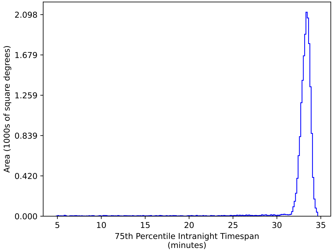
noroll_mjdp180_v3.4_10yrs WFD ug bands: 75th Percentile Intranight Timespan
