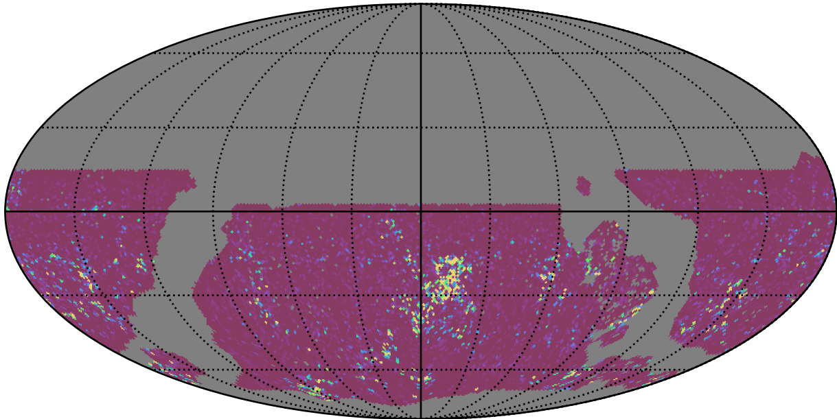
noroll_mjdp180_v3.4_10yrs WFD u band: 75th Percentile Intranight Timespan
