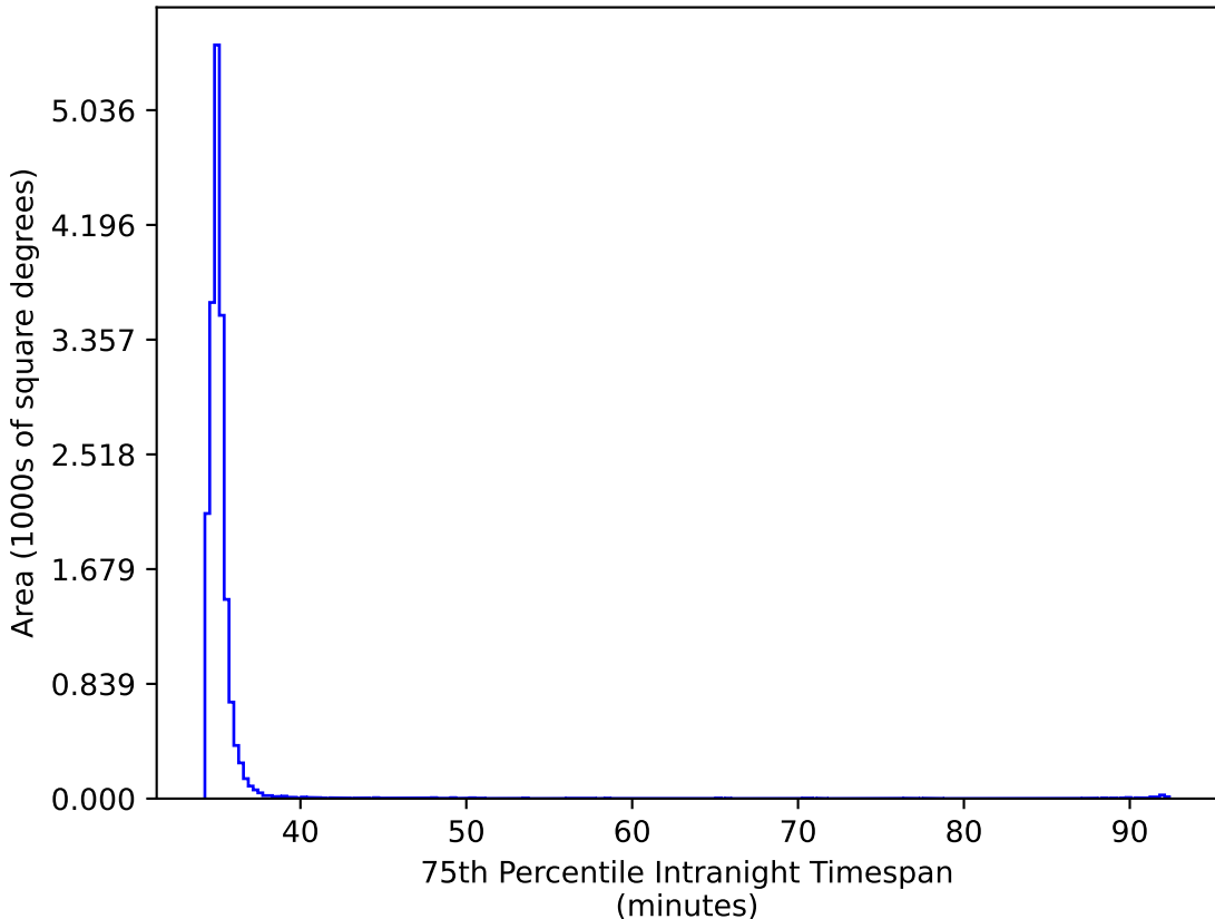
noroll_mjdp180_v3.4_10yrs WFD ri bands: 75th Percentile Intranight Timespan
