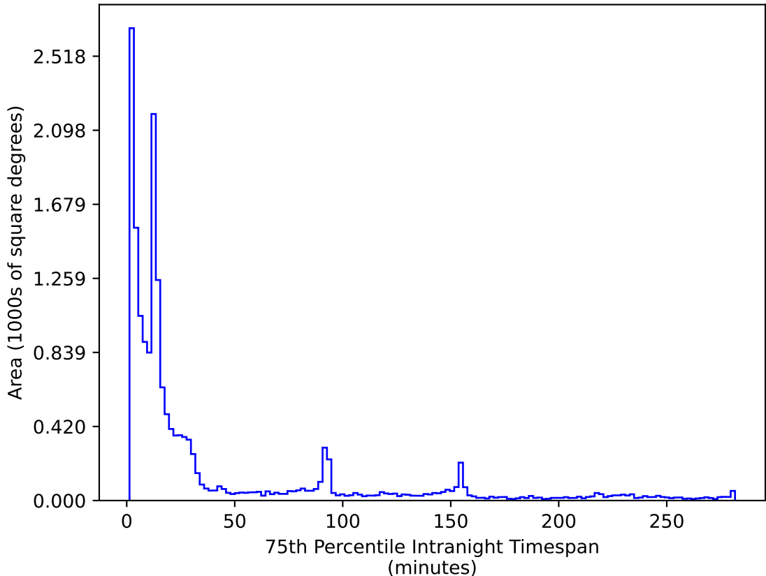
noroll_mjdp180_v3.4_10yrs WFD r band: 75th Percentile Intranight Timespan
