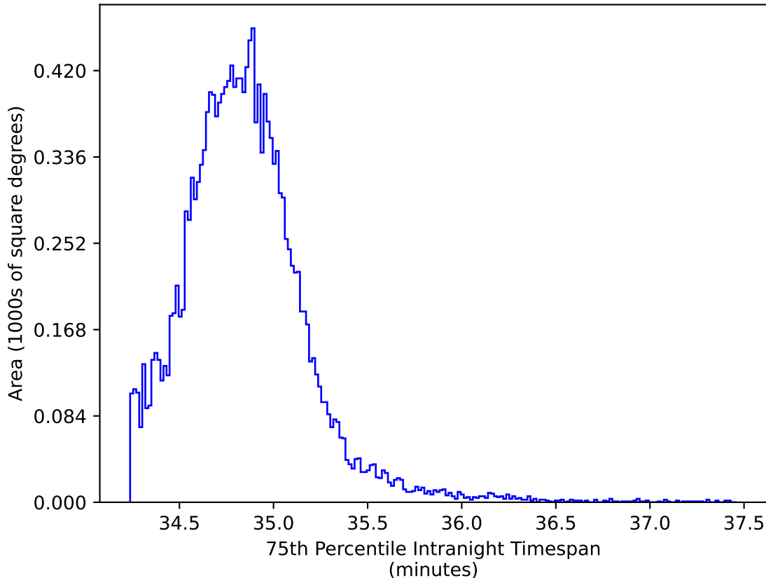
noroll_mjdp180_v3.4_10yrs WFD iz bands: 75th Percentile Intranight Timespan
