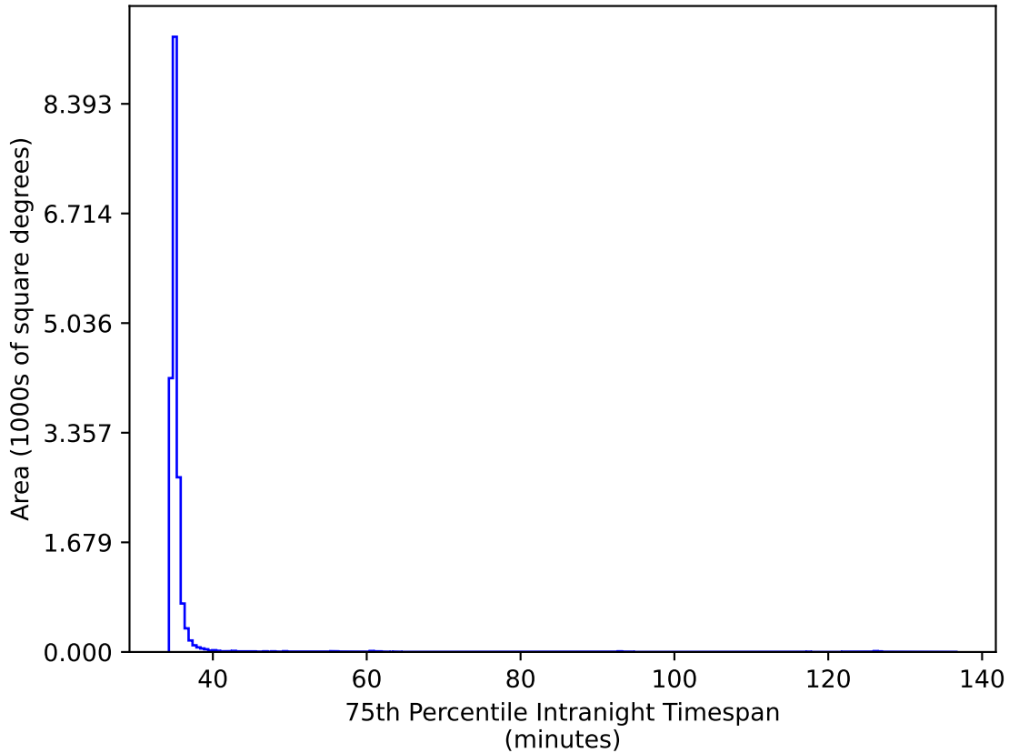
noroll_mjdp180_v3.4_10yrs WFD gr bands: 75th Percentile Intranight Timespan
