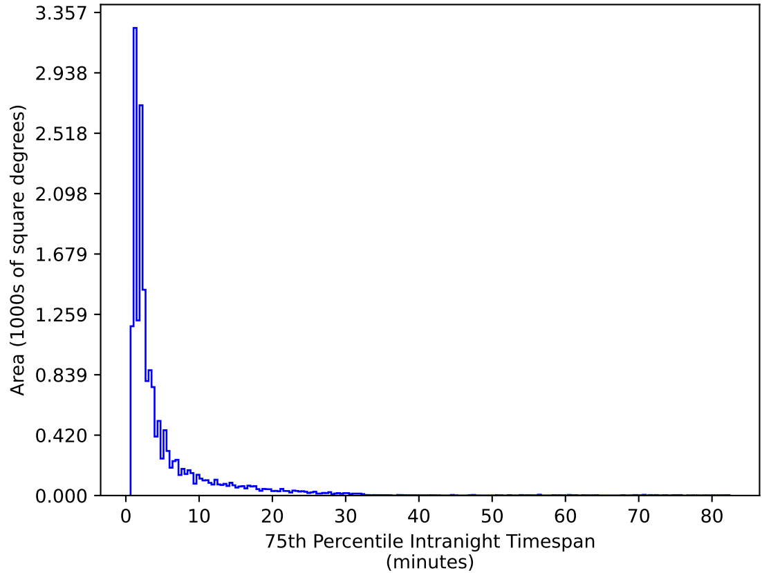
noroll_mjdp180_v3.4_10yrs WFD g band: 75th Percentile Intranight Timespan
