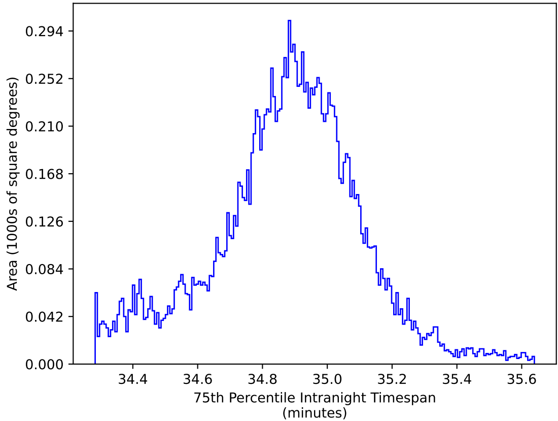
noroll_mjdp180_v3.4_10yrs WFD all bands: 75th Percentile Intranight Timespan
