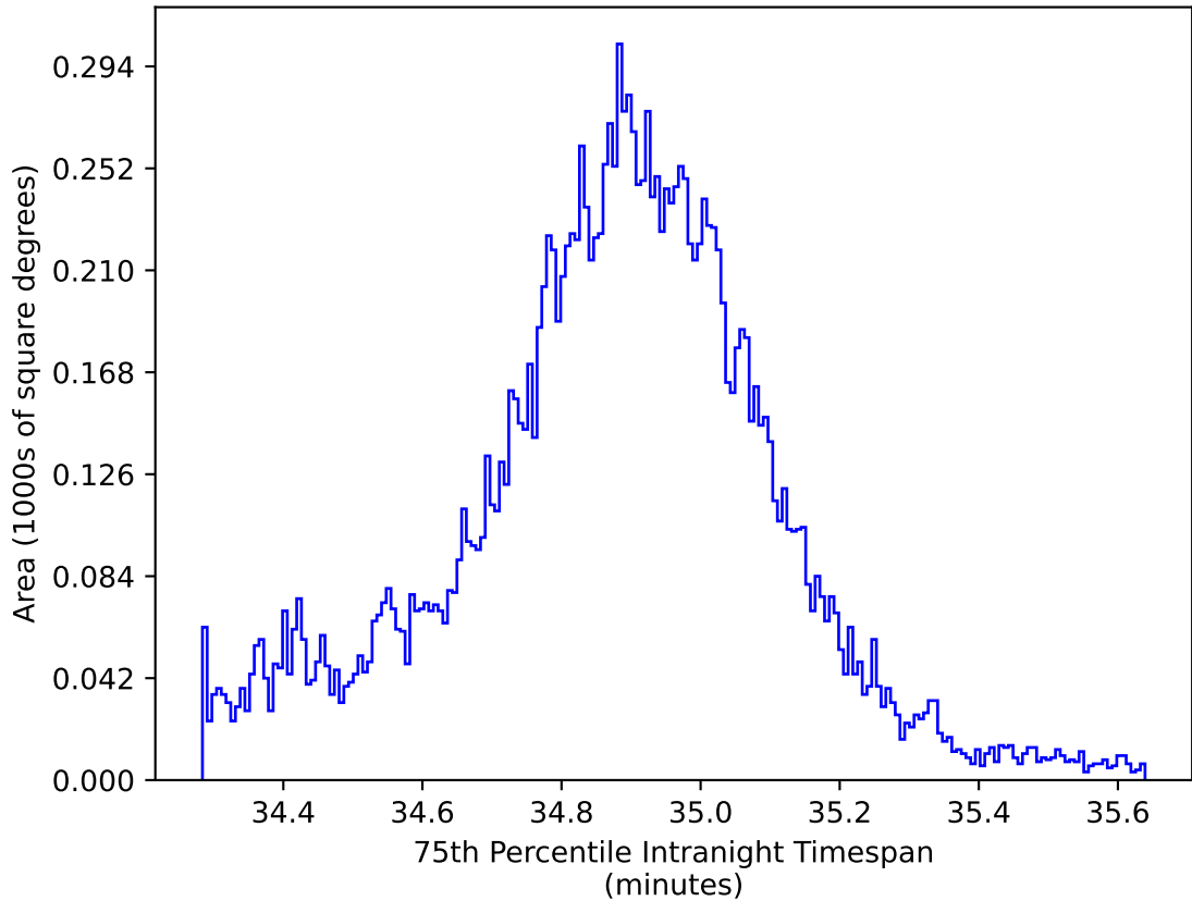
noroll_mjdp180_v3.4_10yrs WFD: 75th Percentile Intranight Timespan
