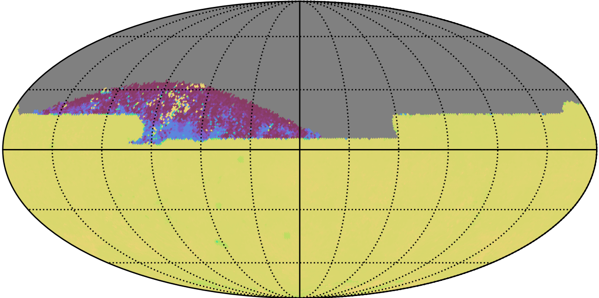
noroll_mjdp180_v3.4_10yrs All sky zy bands: 75th Percentile Intranight Timespan
