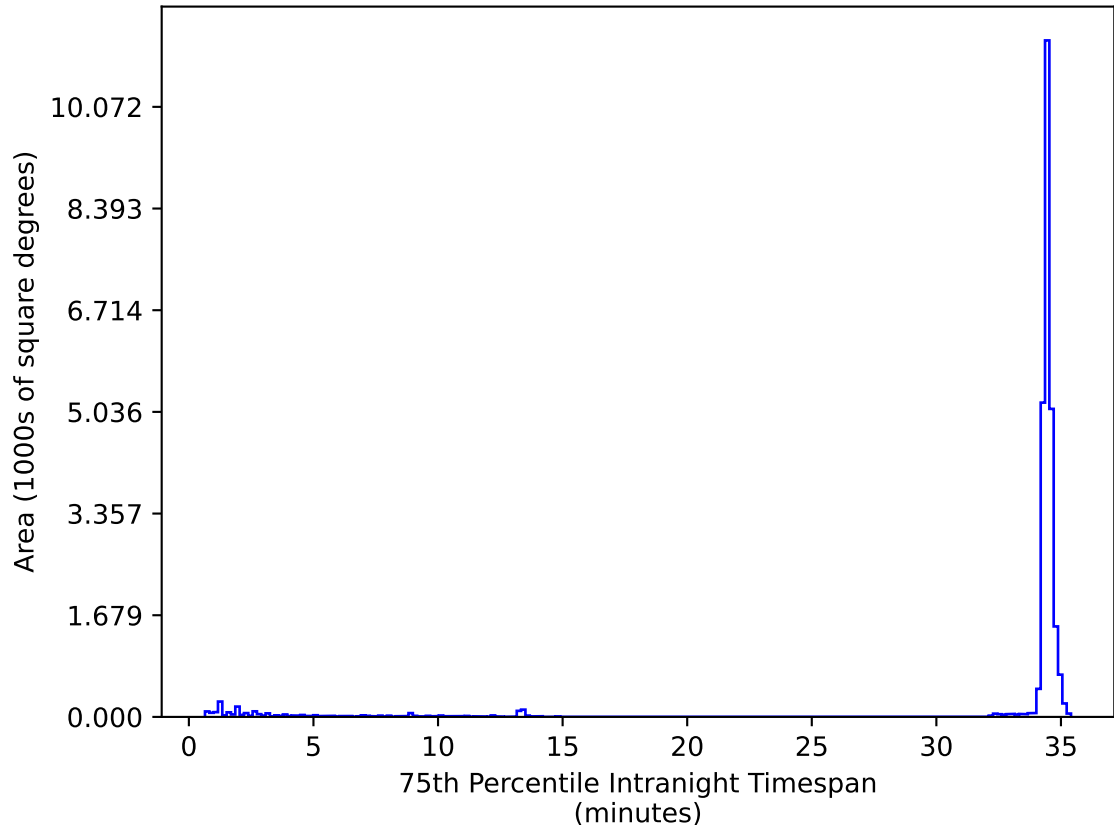
noroll_mjdp180_v3.4_10yrs All sky zy bands: 75th Percentile Intranight Timespan
