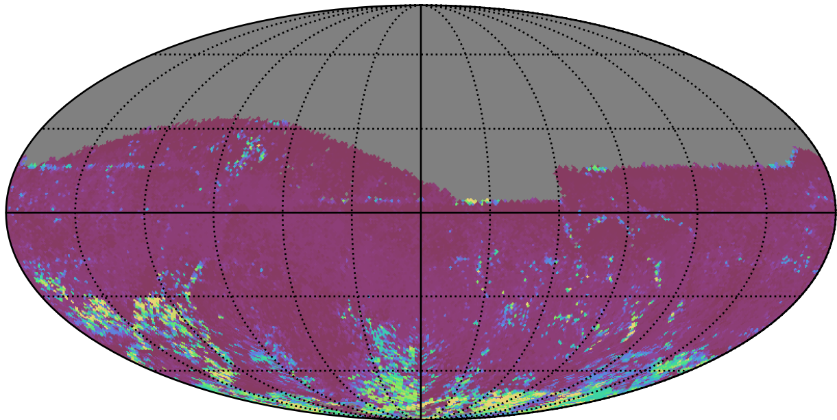
noroll_mjdp180_v3.4_10yrs All sky z band: 75th Percentile Intranight Timespan
