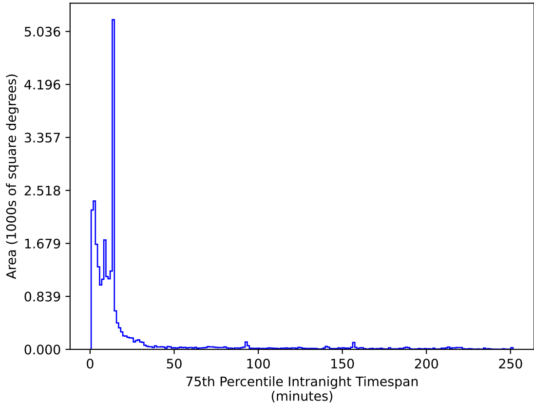
noroll_mjdp180_v3.4_10yrs All sky z band: 75th Percentile Intranight Timespan
