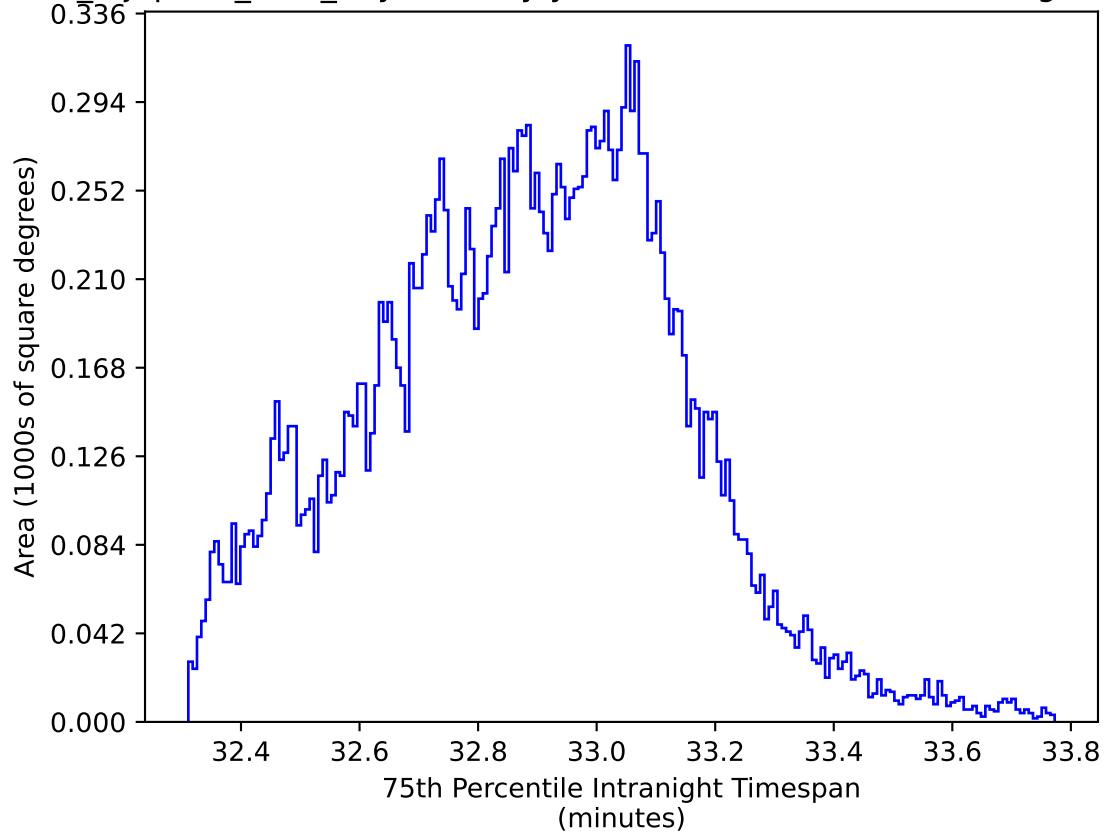
noroll_mjdp180_v3.4_10yrs All sky y band: 75th Percentile Intranight Timespan
