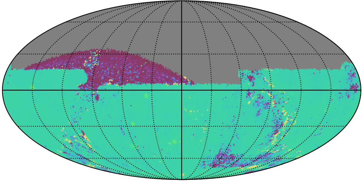
noroll_mjdp180_v3.4_10yrs All sky ug bands: 75th Percentile Intranight Timespan
