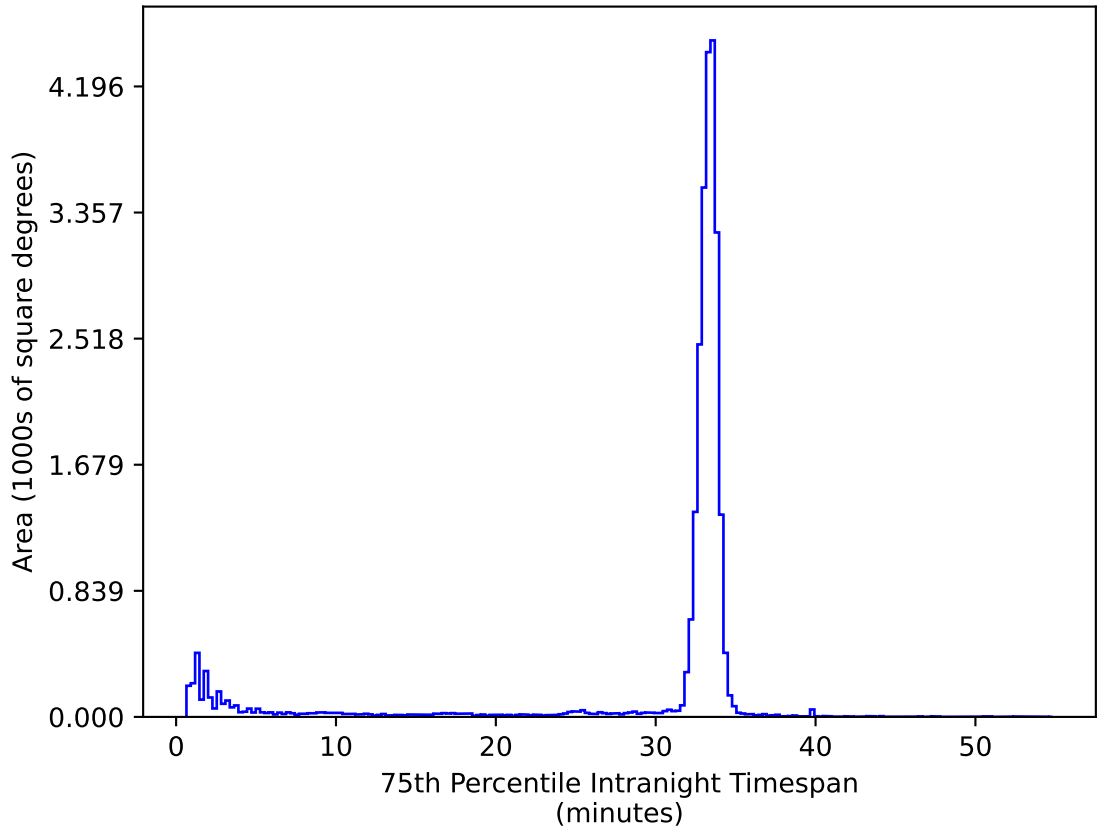
noroll_mjdp180_v3.4_10yrs All sky ug bands: 75th Percentile Intranight Timespan
