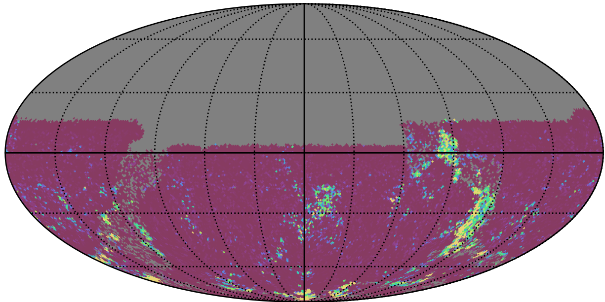
noroll_mjdp180_v3.4_10yrs All sky u band: 75th Percentile Intranight Timespan
